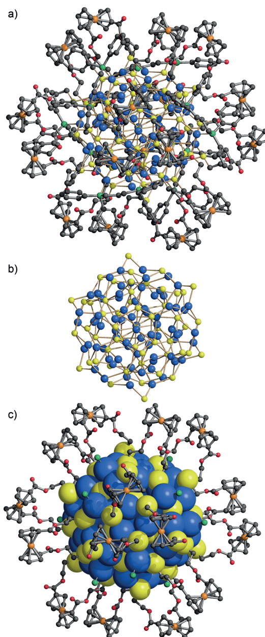
Figure 1. a) Ball-and-stick diagram of the molecular structure of [\text{Ag}_{74}\text{S}_{19}(\text{dppp})_6(\text{fc}(\text{C}(\text{O})\text{OCH}_2\text{CH}_2\text{S})_2)_{18}] ( 1 ). H atoms have been omitted for clarity. b) Ball-and-stick diagram of the \text{Ag}_{74}\text{S}_{55} core of 1 . c) Space-filling diagram of the \text{Ag}_{74}\text{S}_{55} core with the C atoms of \text{dppp} omitted to show the distribution of ferrocenyl ligands in 1 . Atom colors in (a–c): Ag = blue, S = yellow, P = green, O = red, Fe = orange, C = gray.
